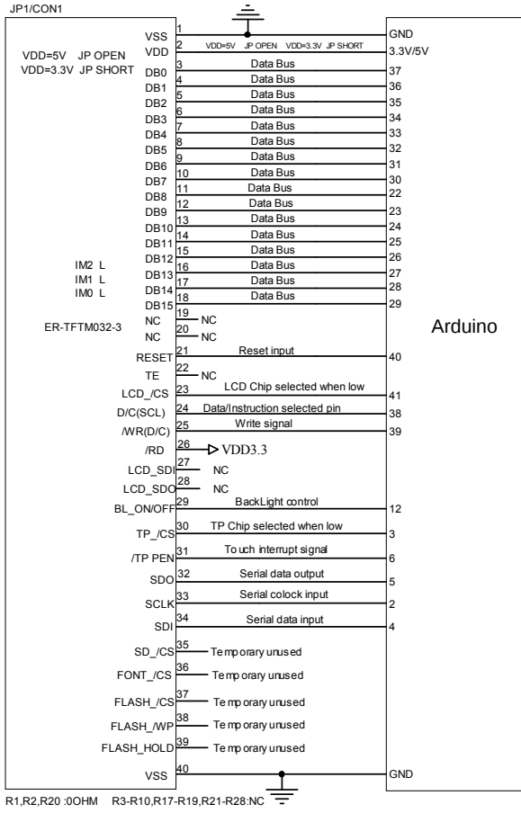
The Parallel 16bit MCU interface(8080 Series II)Reference Example
