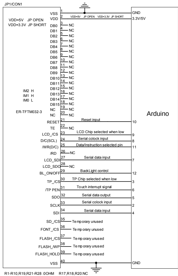
The Serial 4wire SPI MCU interface II Reference Example
