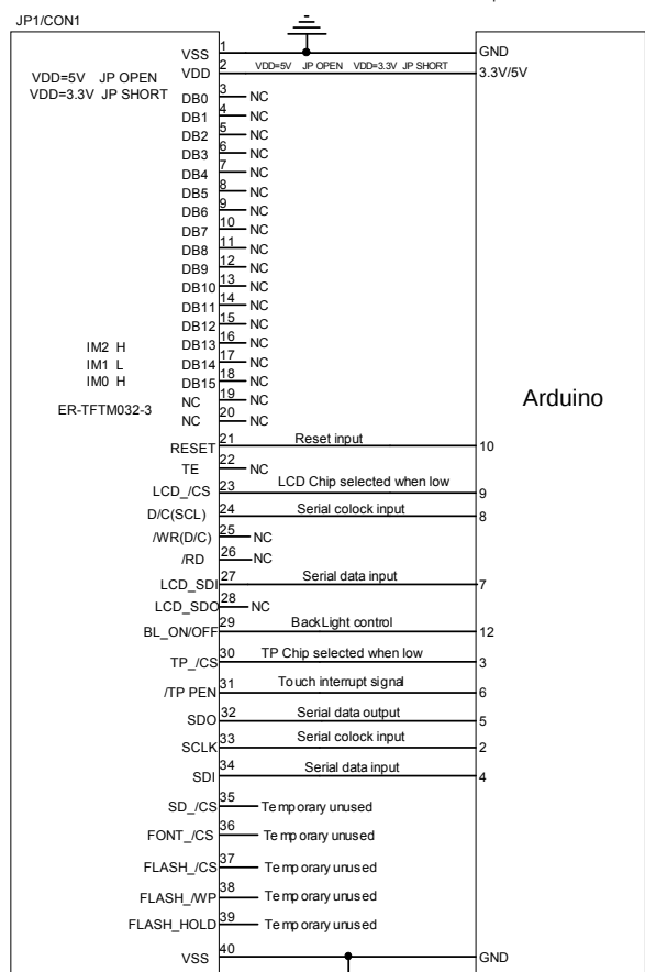
The Serial 3wire SPI MCU interface II Reference Example
