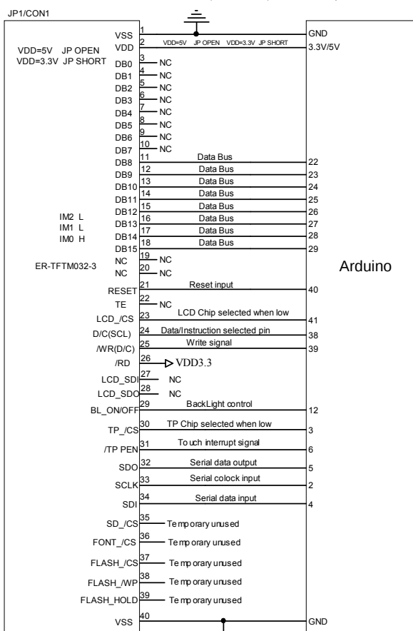
The Parallel 8bit MCU interface(8080 Series II)Reference Example
